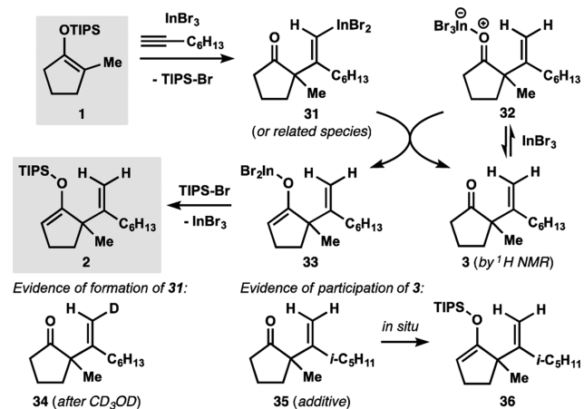
Scheme 3. Proposed Mechanism of the Alkenylation
