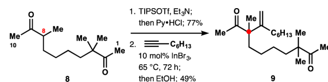
Scheme 2. Synthesis of Diketone 9
